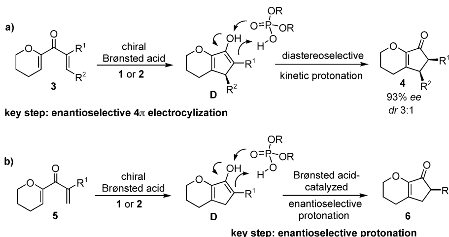
Scheme 2. Origin of enantioselectivity in the Brønsted acid-catalyzed asymmetric synthesis of cyclopentenones: a) for 2,3-disubstituted divinyl ketones enantioselection is induced by an asymmetric electrocyclic ring closure followed by a diastereoselective kinetic protonation and b) in the case of 2-substituted divinyl ketones through the new Brønsted acid-catalyzed enantioselective protonation.
