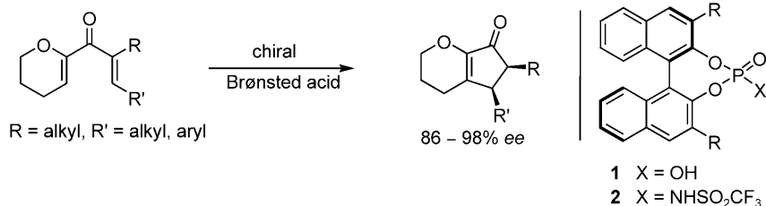
Scheme 1. Enantioselective Brønsted acid-catalyzed Nazarov cyclization.
