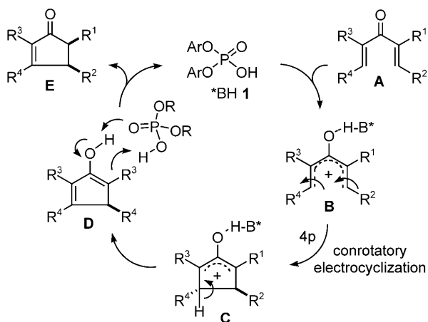
Figure 1. Catalytic cycle of the Brønsted acid-catalyzed Nazarov reaction.
